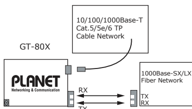
Figure 9: GT-80x Installation
